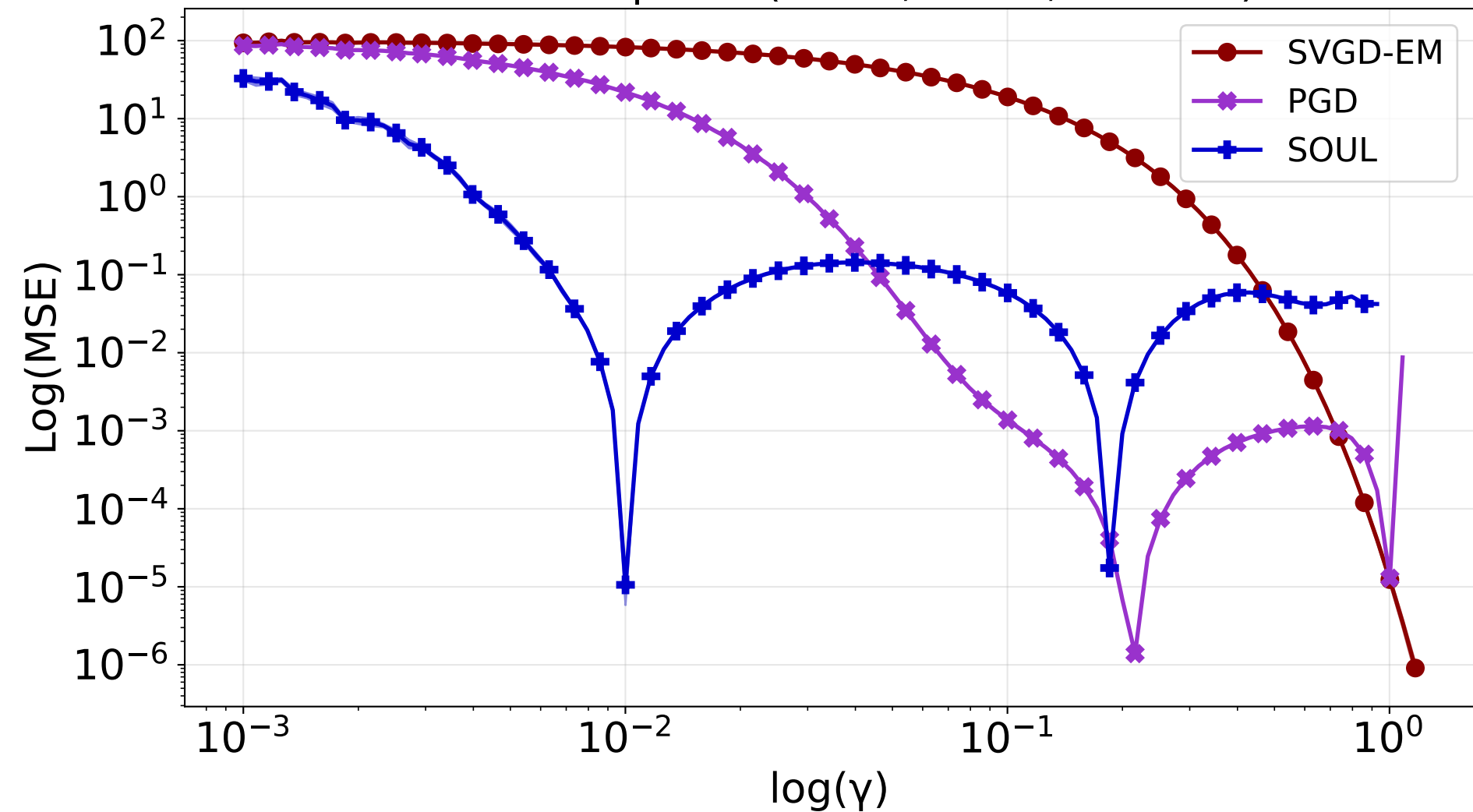
MSE vs Step size (D=20, N=20, K=1000)
